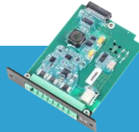
THT ASSEMBLY
