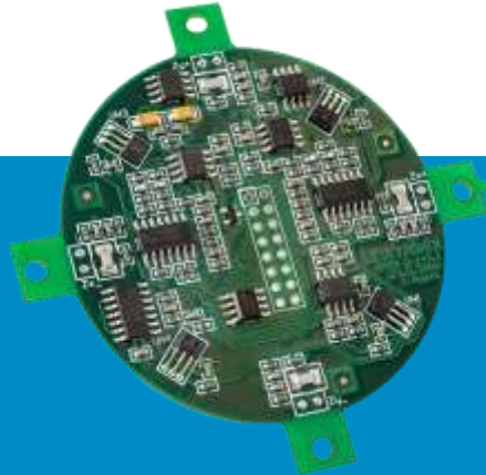
SMD ASSEMBLY
